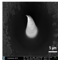
Bending due to excessive coking
