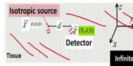
Infinite slab model representation. Image courtesy: Piao et al. 28
